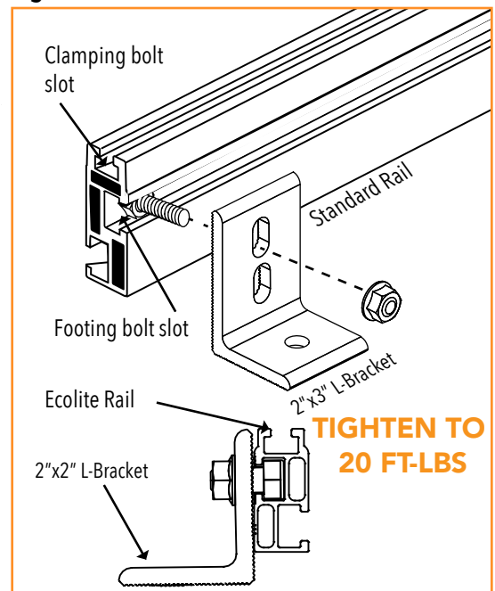
Figure 14. FOOT-TO-RAIL ATTACHMENT
