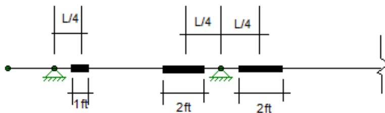
Continuous Span (3 spans or greater)
