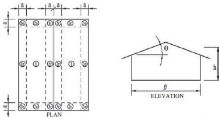
FIGURE 30.3-2D Components and Cladding [ h \leq 60 ft ( h \leq 18.3 m)]: External Pressure Coefficients, ( GC_p ), for Enclosed and Partially Enclosed Buildings—Gable Roofs, 27^\circ < \theta \leq 45^\circ
