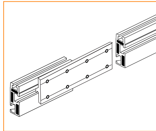
Figure 12. SPLICE BAR ATTACHMENT FOR STANDARD RAILS ONLY
