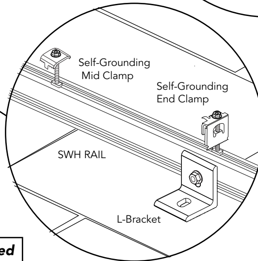
SELF-GROUNDING MID CLAMP & END CLAMP
