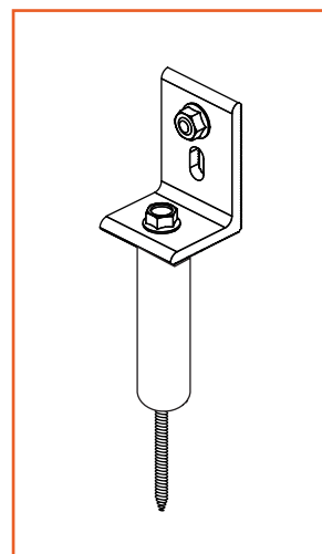
Figure 9. Standoff in conjunction with an L-Bracket.
