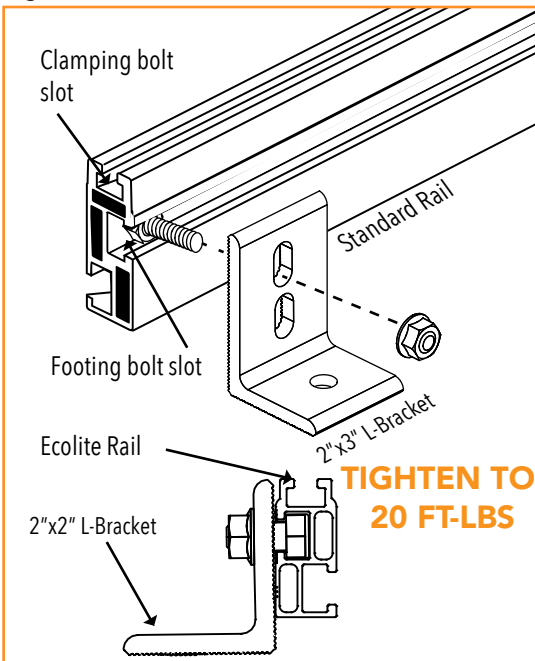
Figure 14. FOOT-TO-RAIL ATTACHMENT
