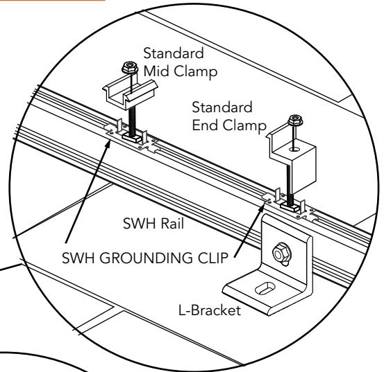
STANDARD MID CLAMP & END CLAMP
