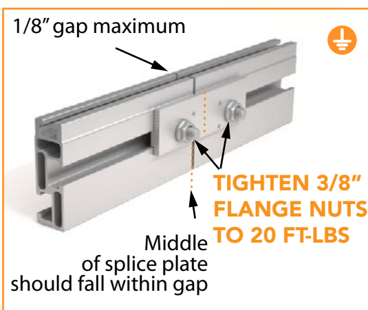
Figure 13. SPLICE PLATE ATTACHMENT FOR STANDARD OR ECOLITE RAILS
